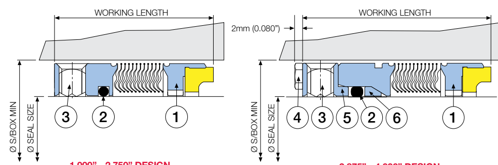
1.000" - 2.750" DESIGN
