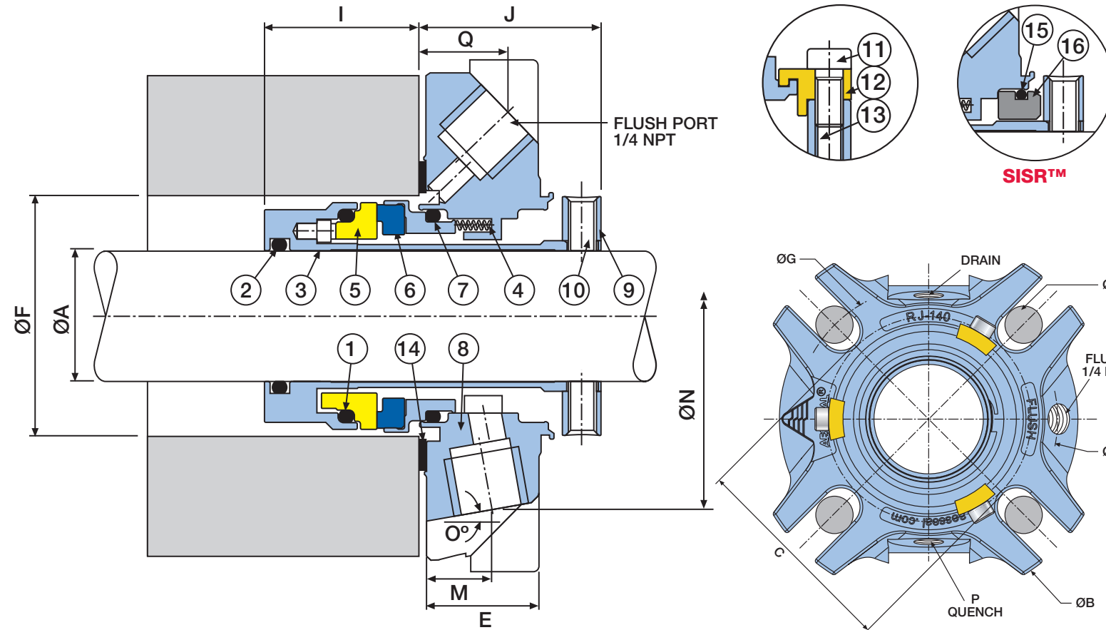
SISS™ - Dimensional Information (mm)
