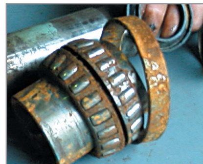
Moisture contaminated bearings
