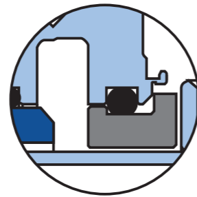
CSSN-R™ Includes optional restriction bush
