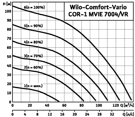
Wilo-Comfort-Vario COR-1 MVIE 7004/VR
