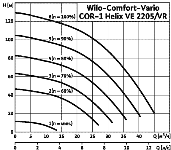
Wilo-Comfort-Vario COR-1 Helix 2205 VE.../VR
